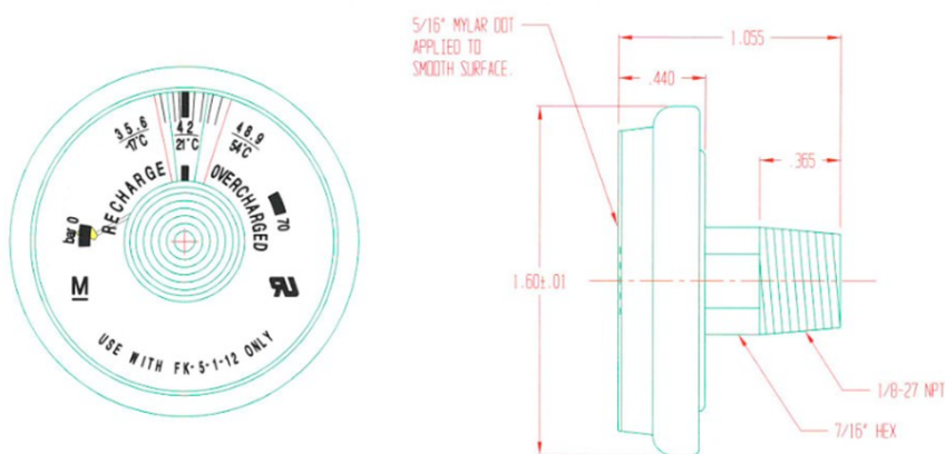
42 Bar Pressure Gauge
