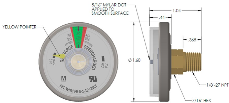
25 Bar Pressure Gauge
