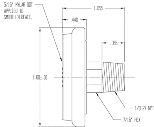
50 Bar Pressure Gauge
